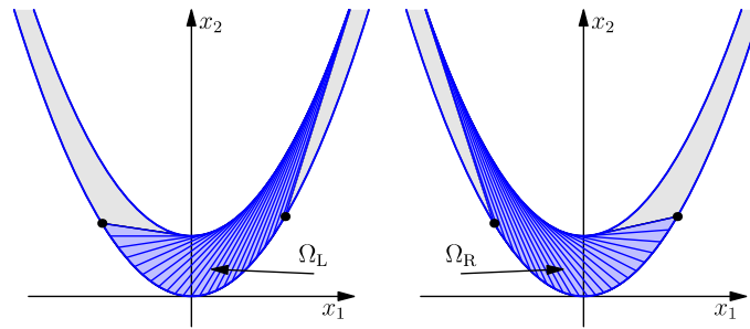
Fig. 1. The domains \Omega_L and \Omega_R .
