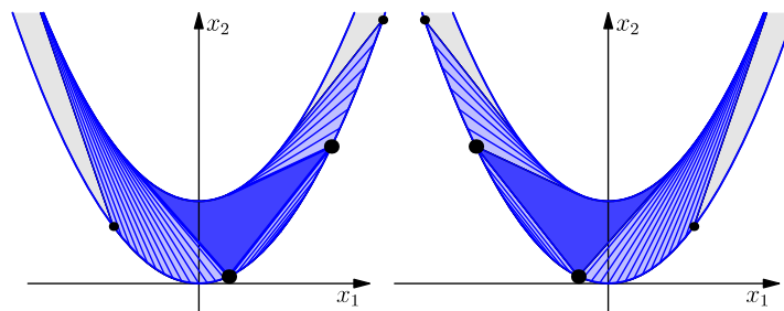
Fig. 4. A right \Omega_{\text{tr},R} and a left \Omega_{\text{tr},L} trolleybuses.
